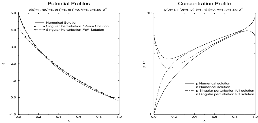
FIG. 6. The comparison of the numerical solution and the singular perturbation full solution for the general boundary condition BC2 with a large V . The same convention is used as Fig. 5
