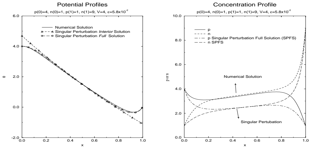
FIG. 7. The comparison of the numerical solution and the singular perturbation full solution for the general boundary condition BC3 with a large V . The same convention is used as Fig. 5
