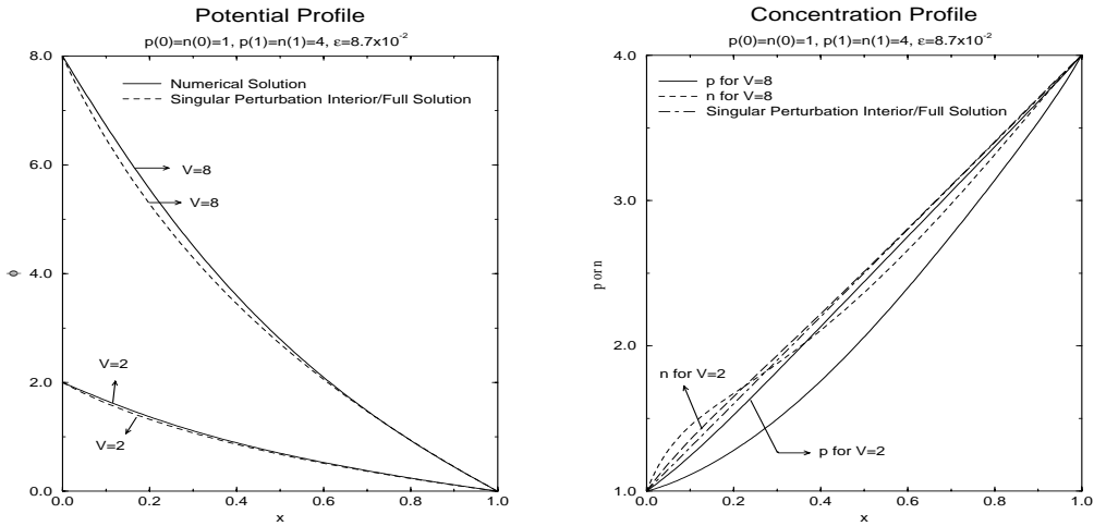
FIG. 2. The electric potential profile and concentration profiles for the simple boundary condition, Case 1. Dimensionless concentration and potential units employed. Original units of 100 mM and 25 mV, resp.
