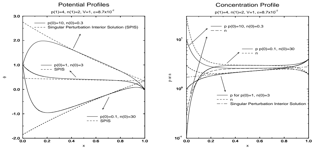
FIG. 3. The comparison of the numerical solution and the singular perturbation interior solution for the general boundary conditions BC1 and BC4.
