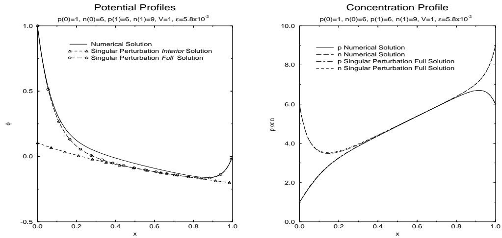
FIG. 5. The comparison of the numerical solution and the singular perturbation full solution for the general boundary condition BC2.
